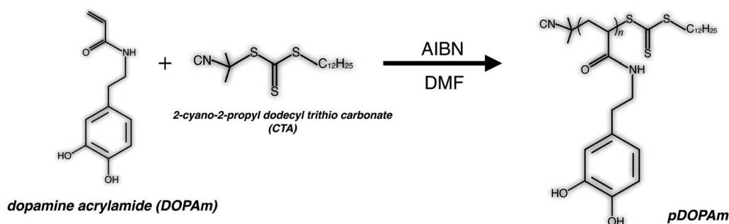
Scheme 1 Synthesis of poly(dopamine acrylamide) (pDOPAm).
