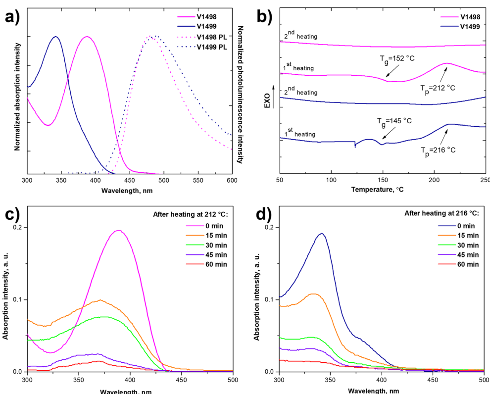
Fig. 1 (a) UV-vis absorption (solid line) and photoluminescence (dashed line) spectra of thin films of V1498 and V1499 ; (b) DSC first and second heating curves of HTMs (scan rate 5^\circ\text{C min}^{-1} , \text{N}_2 atmosphere); cross-linking experiment of V1498 (c) and V1499 (d) films. The absorption of the solutions, prepared by dipping spin-coated and cured at adequate temperatures HTM films into THF for the respective duration.
