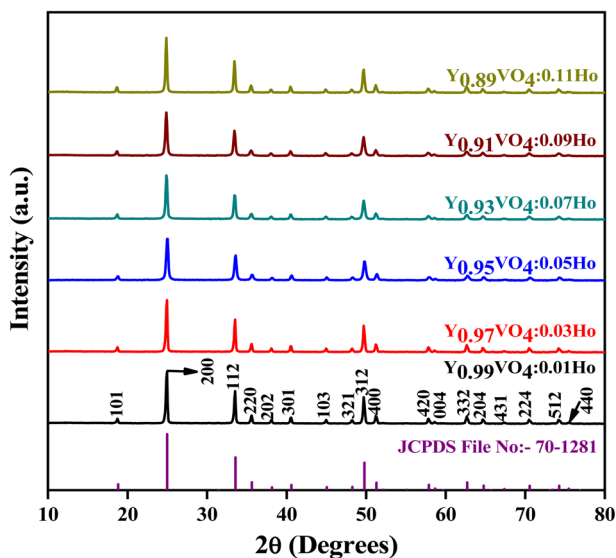
Fig. 3 Powder XRD patterns of \text{Y}_{1-x}\text{VO}_4:x\text{Ho}^{3+} phosphors.
