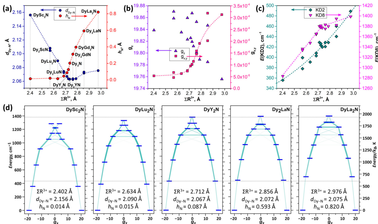
Fig. 5 (a) Dy–N bond lengths ( d_{\text{Dy-N}} ) and M_3N pyramid height (elevation of N above the plane of metal atoms, h_N ) in DFT-optimized \text{DyM}_2\text{N}@C_{80} and \text{Dy}_2\text{MN}@C_{80} molecules ( M = \text{Sc}, \text{Lu}, \text{Y}, \text{La}, \text{Gd} ) plotted versus the sum of Shannon's ionic radii of metals in the M_3N cluster ( \Sigma R^{3+} ). (b) Components of the pseudospin g -tensor, g_z and g_{x,y} (root mean square of g_x and g_y ) for the \text{Dy}^{3+} ground state Kramers doublet (KD1) in the same set of molecules. (c) The energy of the first excited KD (KD2) and the total ligand-field splitting (KD8) in the same set of molecules. Dashed lines in (a) and (b) are a spline interpolation added to guide the eye; in (c), the dashed line for E(\text{KD2}) is a quadratic fit. (d) \text{Dy}^{3+} ligand-field splitting with transition probabilities in selected M_3N@C_{80} molecules along with their \Sigma R^{3+} , d_{\text{Dy-N}} , and h_N parameters; dotted lines are guides to the eye and mark the KD2 and KD8 energies in \text{Dy}_2\text{N}@C_{80} . Ligand-field splitting and pseudospin g -tensor parameters used in (b–d) are computed ab initio at the CASSCF/RASSI-SO level using DFT-optimized molecular structures.
