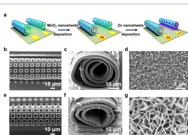
Fig. 2 Manufacture of mesostructured Swiss-roll microelectrodes. (a) Schematic of the Zn– \text{MnO}_2 Swiss-roll microbattery fabrication process. (b) Top (b) and side view (c) SEM images of mesostructured Swiss-roll microcathode. (d) Magnified SEM image of the \text{MnO}_2 morphology. Top (e) and side (f) view of mesostructured Swiss-roll microanode. (g) Magnified SEM image of the Zn nanosheet morphology.
