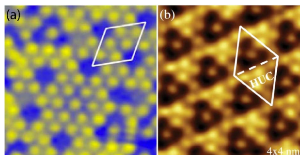
Fig. 12 STM images of the 2(\sqrt{3} \times 2\sqrt{3})R30^\circ (a) and (4 \times 4) \text{Si}/\text{Ag}(111) reconstruction (b) after hydrogenation exposure. In (a) the rhombus corresponds to the pristine 2(\sqrt{3} \times 2\sqrt{3})R30^\circ unit cell, while in (b) it corresponds to a shift of the pristine (4 \times 4) unit cell. Adapted with permission from ref. 66, Copyright 2015 by the American Physical Society and with permission from ref. 81, Copyright 2015 American Chemical Society.
