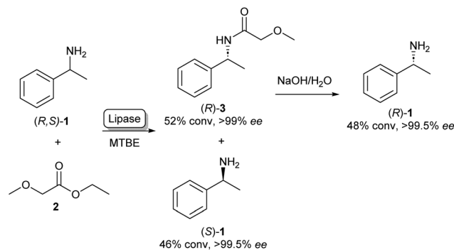
Scheme 1 Lipase catalysed kinetic resolution of amines: selective acylation of (R,S) -1 using lipase in MTBE (methyl tert -butyl ether) yielding (S) -1. Basic hydrolysis of amide 3 yields (R) -1. 21
