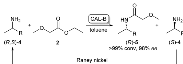
Scheme 2 CAL-B/RANEY® nickel catalysed dynamic kinetic resolution of 4 yielding enantiopure (R) -5. CAL-B selectively acylates (R) -4 while the unreacted (S) -4 is converted back to the racemate by the RANEY® nickel catalyst. 23
