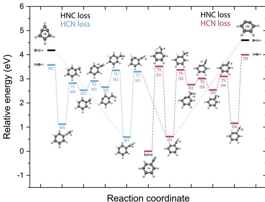
Fig. 6 Potential energy surface for the fragmentation to both o -benzynes + (red pathway) and bicyclic m -benzynes + (blue pathway) from benzonitrile + leading to either HCN loss (O-pathway, red), (M-pathway, blue) or HNC loss (black energy levels, solid lines). The energies are calculated at the B3LYP-GD3/N07D level of theory and are corrected for the zero-point vibrational energy.
