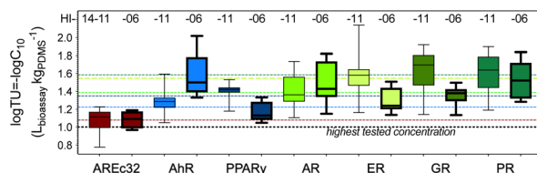
Fig. 2 Comparison of toxic units TU for cytotoxicity between the different cell lines and the two animals – HI-14-11 (thin lines) and HI-14-06 (thick lines), sorted according to increasing mean TU (dotted lines with matching colours, mean of all data from both animals).
