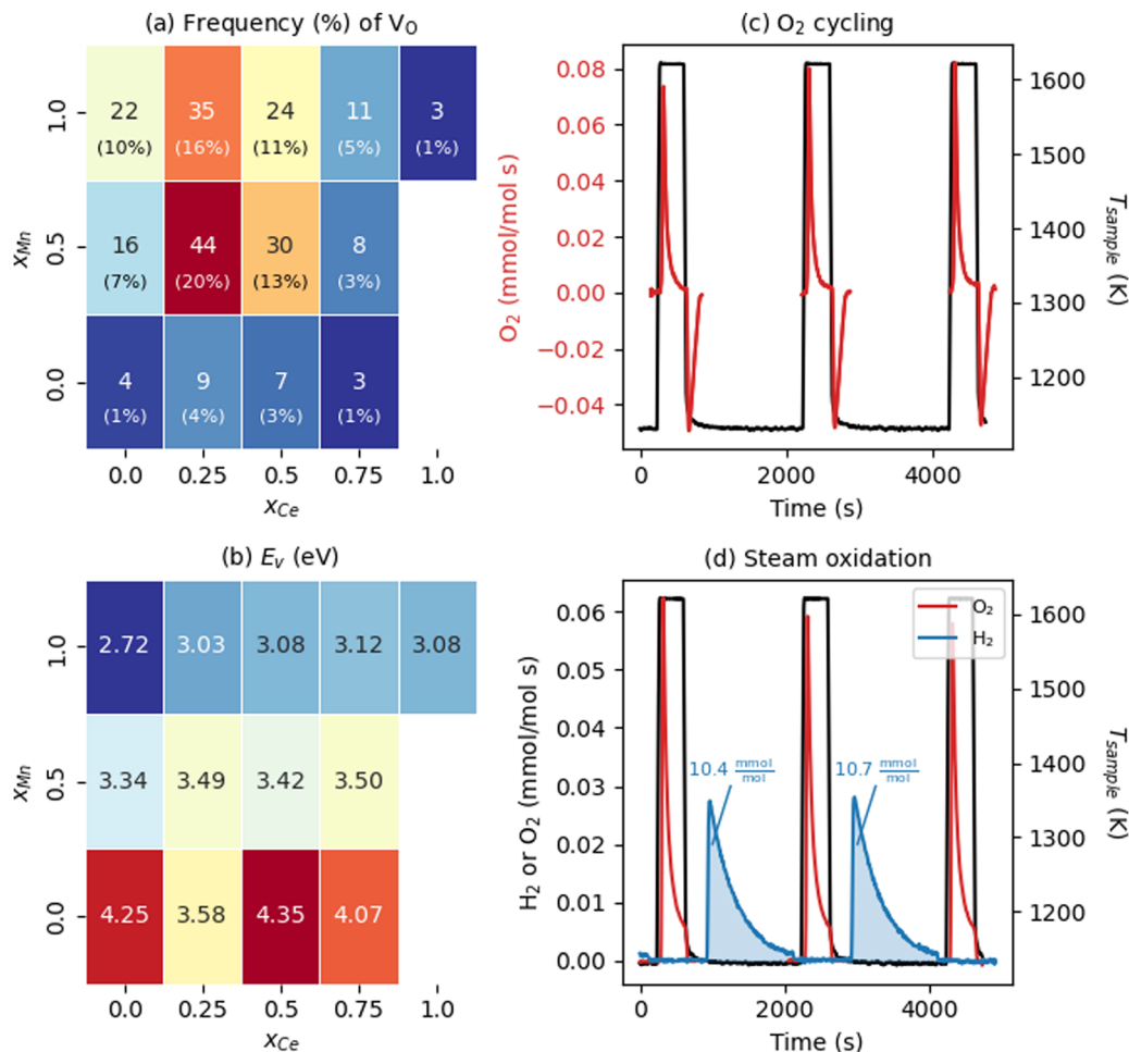
Fig. 2 Water-splitting properties of CCTM2112. (a) Frequency (color of and text in rectangles) and probability (percentages in parentheses rounded to the nearest integer) of all unique NN V_{\text{O}} environments in the calculated CCTM2112 360-atom cell (and, in Table S6, ESI† for the random alloy), with dark red and dark blue shading indicating higher- and lower-frequency environments, respectively. (b) NN- V_{\text{O}} -environment dependence of calculated E_v in CCTM2112. Color of and text in rectangles correspond to E_v in eV, where the minimum E_v = 2.72 eV is dark blue and maximum E_v = 4.35 eV is dark red. (c) \text{O}_2 evolution rate normalized to mole atoms in CCTM2112 (see ESI,† Section S5 for definition) measured as a function of time during heating and cooling between 1123 K and 1623 K in a constant background of 2000 ppm oxygen. (d) \text{O}_2 and \text{H}_2 evolution rates normalized to mole atoms in CCTM2112 measured as a function of time during two successive redox cycles where the sample temperature is raised to 1623.15 K while sweeping with high purity Ar, followed by exposure to 40 vol% \text{H}_2\text{O} in Ar at 1123.15 K. The area under the gas evolution features in (c) and (d) is used to quantify the redox capacity of CCTM2112 during oxygen and steam oxidation.
