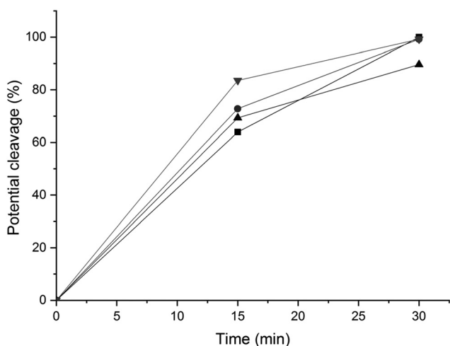
Fig. 11 Potential conversion of the \beta\text{-O-4' } (\beta) ( \blacksquare ), \beta\text{-O-4' } (\alpha) ( \bullet ), \beta\text{-5'} ( \blacktriangle ) and 5\text{-5'} ( \blacktriangledown ) environments according to the HMBC spectra with the integration of the signals at (4.19, 146.77 ppm), (4.97, 108.42 ppm), (5.08, 110.29 ppm) and (6.89, 124.09 ppm) respectively.
