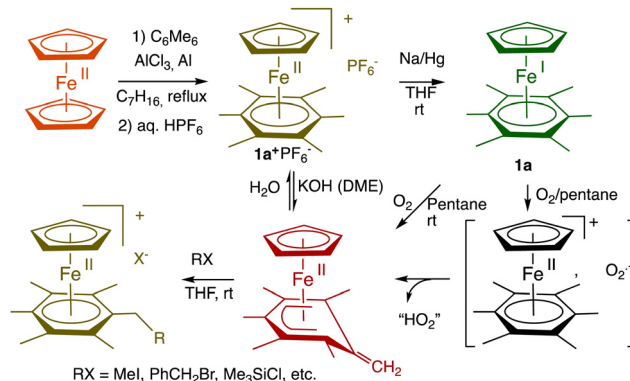
Scheme 1 Synthesis and reaction with \text{O}_2 of the 19-electron \text{Fe}(\text{I}) complex 1a . Due to the large difference (about 1 V) between the two redox systems \text{Fe}(\text{I})/\text{Fe}(\text{II}) and \text{O}_2/\text{O}_2^{\bullet-} , electron transfer from \text{Fe}(\text{I}) to \text{O}_2 is very exergonic and fast, followed by deprotonation by \text{O}_2^{\bullet-} within the intermediate ion cage (from \text{O}_2^{\bullet-} EPR). 14,15 In THF, this cage superoxide reaction is totally inhibited by \text{NaPF}_6 due to ion exchange between the two ion pairs [\text{Fe}(\text{II})^+, \text{O}_2^{\bullet-}] and [\text{Na}^+, \text{PF}_6^-] , 16 (for a review of salt effects, see ref. 17) which is reminiscent of the function of superoxide dismutase enzyme. 18
