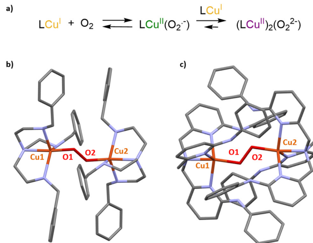
Fig. 4 (a) Formation of primary and secondary O 2 adducts arising from O 2 activation in open Cu(I) complexes. XRD structures of [(Cu(L)) 2 (O 2 )] peroxo dimers observed upon O 2 activation in (b) Cu I (TREN) and (c) Cu I (TPA) derivatives.
