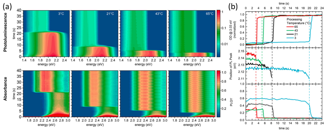
Fig. 25 Evolution of (a) normalized PL (top) and absorbance (bottom) spectra of P3HT spin-coated from CB at different temperatures. (b) Evolution of optical density (OD) of the absorption band from aggregated P3HT, peak position of emission maxima, and PLQY during film formation at different temperatures. Adapted with permission. 91 Copyright 2018, American Chemical Society.
