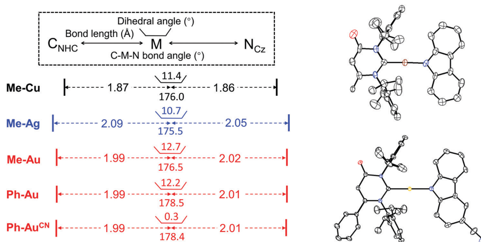
Fig. 2 Critical crystallographic data from X-ray single crystal diffraction measurements, C_{NHC} denotes the carbene carbon and N_{Cz} is the carbazolyl nitrogen. Thermal ellipsoid figures of Me-Cu (top) and Ph-Au CN (bottom).
