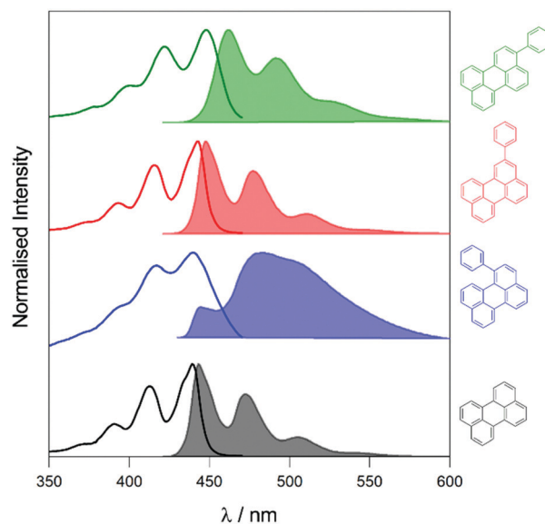
Fig. 1 UV-Visible absorption (solid line) and emission (solid filled, \lambda_{\text{exc}} = 410\text{ nm} , [perylene] = 1\text{--}2\ \mu\text{M} ) spectra of perylene derivatives in toluene. Structures of the compounds are displayed in the colour corresponding to their spectra.
