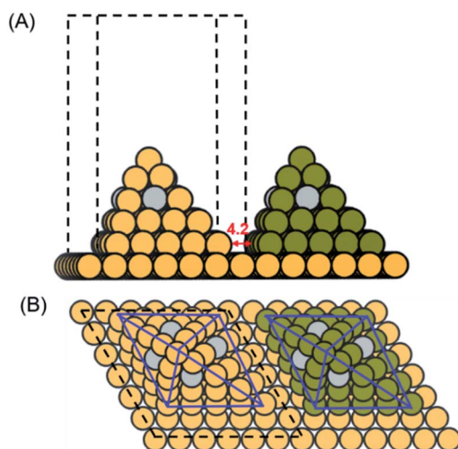
Fig. 1 (A) Side view and (B) top view of the atomic structure of Ag-doped Cu-DAN. The computational model is constructed based on a 6 \times 6 \times 1 Cu (111) surface with a 4.2 \text{\AA} space between adjacent Cu nanopyramids (in green) to represent the dense-array, with one Ag atom doped to each sidewall. Colour codes: Cu, orange and green; Ag, silver. Solid blue lines serve as visual guides to show the Cu atoms on the edge. Black dashed lines depict the unit cell.
