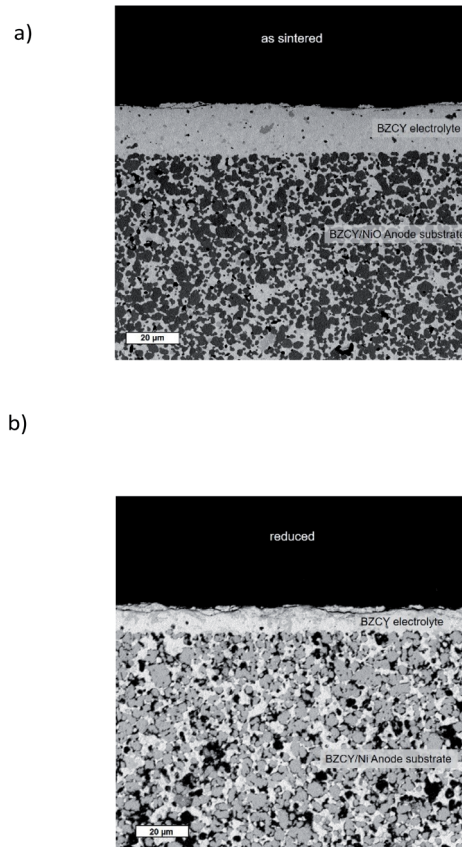
Fig. 11 SEM cross sections of final sintered BZCY–NiO/BZCY bi-layer assemblies at 1500 °C for 6 h. (a) Unreduced, (b) reduced in Ar/H 2 at 900 °C.
