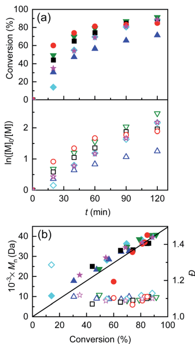
Fig. 4 (a) Kinetic plots and (b) evolution of M_n and D vs. conversion for eATRP of n BA in DMF + 0.1 M Et 4 NBF 4 , T = 45 °C, performed using a Cu/Al electrode pair under various conditions. (■) Potentiostatic electrolysis at E_{app} = E_{1/2} - 0.06 V (Table 2, entry 5); (●) CGE, Q = 1.66 C (Table 3, entry 7); (▲) PGE, Q = 1.66 C (Table 4, entry 1), (▼) PGE, Q = 0.83 C (Table 4, entry 2); general conditions: n BA/EBiB/Cu(OTf) 2 /Me 6 TREN/Et 4 NBr = 349/1/0.1/0.3/0.1, C_{nBA} = 3.49 M. (♦) PGE, Q = 0.83 C n BA/EBiB/Cu(OTf) 2 /Me 6 TREN/Et 4 NBr = 349/1/0/0.3/0.1, C_{nBA} = 3.49 M (Table 4, entry 4); (★) PGE, Q = 0.83 C, n BA/EBiB/Cu(OTf) 2 /Me 6 TREN/Et 4 NBr = 349/1/0.01/0.3/0.1, C_{nBA} = 3.49 M (Table 4, entry 5). The straight line in (b) stands for the theoretical molecular weights.
