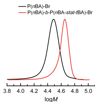
Fig. 5 Molecular weight distribution of P( n BA) 288 -Br macroinitiator ( M_n = 37.0 kDa and D = 1.11 , conv. BA = 83%) and P( n BA) 288 - b -P( n BA 40 - stat -tBA 56 )-Br copolymer ( M_n = 50.6 kDa and D = 1.06 , conv. tBA = 25%, conv. BA = 94%) produced by PGE eATRP of n BA and n BA + t BA at T = 45 °C in DMF + 0.1 M Et 4 NBF 4 . t BA was added after 1 h of n BA polymerization under the following conditions: n BA/EBiB/Cu(OTf) 2 /Me 6 TREN/Et 4 NBr = 349/1/0.1/0.3/0.1, C_{nBA} = 3.49 M.
