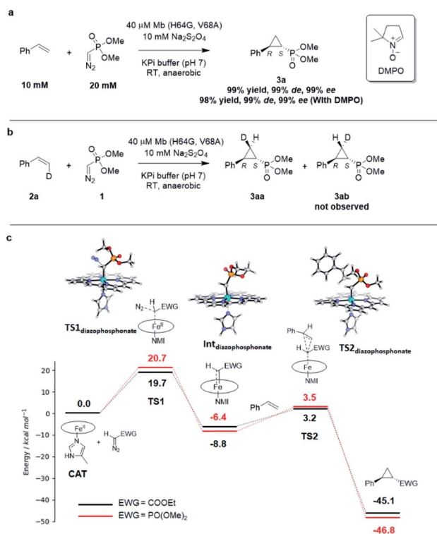
Fig. 3 (A) Radical trapping experiment with styrene and dimethyl (diazomethyl)phosphonate. (B) Enzymatic cyclopropanation reaction with cis -β-deutero-styrene. (C) Gibbs free energy diagram for the heme-catalyzed styrene cyclopropanation reaction with dimethyl (diazomethyl)phosphonate ( 1 ) and EDA. Molecular models of key TS and intermediates in the reaction pathway with 1 are shown. \Delta G values calculated based on the UB3LYP/6-311G** + SDD//UB3LYP-D3BJ/def2-TZVP + SDD method. See Table S8† for further details. NMI = 5-methyl-imidazole.
