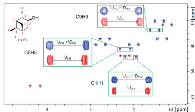
Fig. 6 Overlaid [ 1 H, 13 C]-CLIP-HSQC spectra of (+)-IPC in the isotropic phase (red contours) and 5% OPA-4 alignment medium (anisotropic, blue contours).
