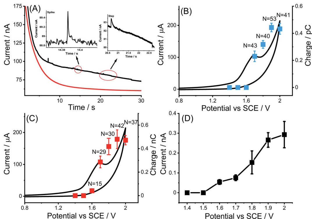
Fig. 2 (A) Chronoamperograms of a carbon micro-disc electrode ( d = 33 \mu\text{m} ) immersed in a 0.1 M KNO 3 (pH = 6.4) solution containing 0.01 g L -1 MWCNTs (black line) or not (red line) at a potential of 1.90 V vs. SCE. The inset is an enlarged view of impact spike and step at 1.90 V; overlay of the plot of average impact spike charge (B) and step charge (C) as a function of applied potentials with the cyclic voltammogram (black line) of MWCNTs modified GCE; (D) average step currents observed as a function of applied potential in 0.1 M KNO 3 (pH = 6.4) containing 0.01 g L -1 MWCNTs (the error bars are derived from \text{SD}/(n)^{1/2} , where SD is the standard deviation and n is the number of the spikes or steps).
