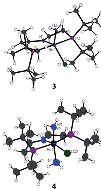
Fig. 1 Solid-state structures of Re–amide complex 3 and Re(NH_3)_2 complex 4 ( BARF_4 ion omitted) with thermal ellipsoids at 50% probability.
