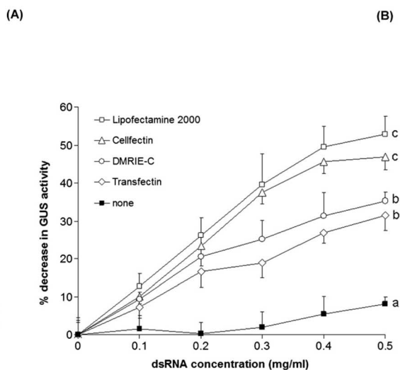
Fig. 9 Cationic liposomes as efficient transfection agents in RNAi. (A) The cationic lipids/liposomes are amphiphilic molecules with overall positive charge. They bind to the nucleic acid as well as cell membranes with electrostatic interactions. The lipid based complex enters the target cell through endocytosis and is subsequently released into the cytoplasm. If the exogenous nucleic acid to be supplied is a DNA, then it needs to be transported into the nucleus while in case of a mRNA molecule it stays within the cytoplasm. 125 (B) A study by Whyard et al. (2009) 119 demonstrated the effect of different transfection agents and dsRNA concentration on the GUS gene in the gut of D. melanogaster larvae. The transfection agents when each coupled with a GUS-dsRNA concentration of 0.5 mg ml -1 brought about an improved silencing effect on the GUS gene as compared to the dsRNA alone. Among all the combinations, Lipofectamine 2000 coupled dsRNA showed maximum GUS silencing activity (more than 50%) as evident from the graph. (Fig. 9B has been reproduced from Whyard et al. (2009) 119 with permission from Elsevier, copyright 2009).
