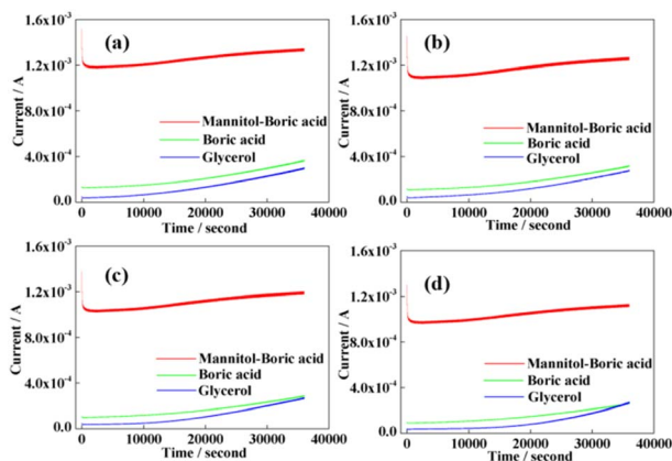
Fig. 5 (a) Comparison of a pure glycerol solution, pure boric acid, and mannitol combined boric acid of the same concentration in 10^{-1} mol L^{-1} , (b) 10^{-2} mol L^{-1} , (c) 10^{-3} mol L^{-1} , and (d) 10^{-4} mol L^{-1} .
