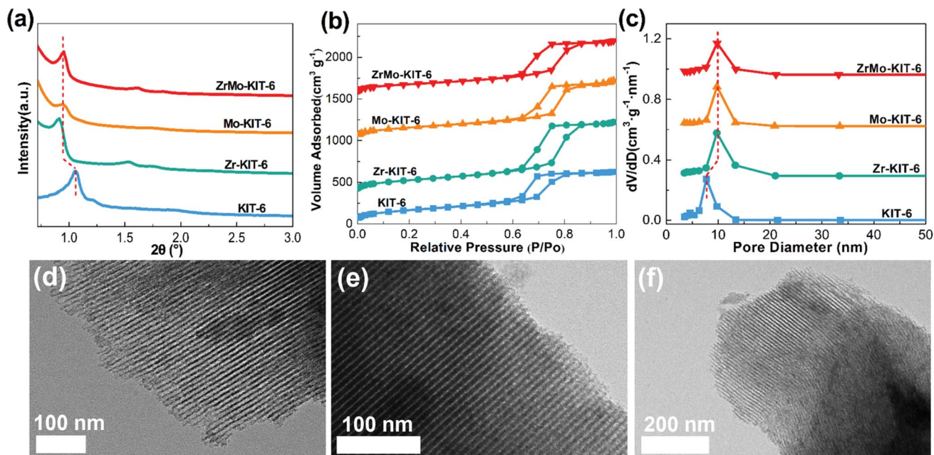
Fig. 1 (a) SXR D patterns, (b) isotherms, and (c) pore size distributions of KIT-6, Zr-KIT-6, Mo-KIT-6, and ZrMo-KIT-6. TEM images of (d) Zr-KIT-6, (e) Mo-KIT-6, and (f) ZrMo-KIT-6.
