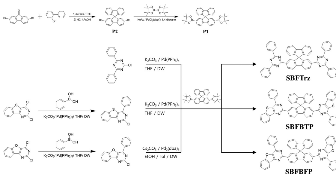
Scheme 1 Synthesis process of SBFTz, SBFBTP and SBFBFP.
