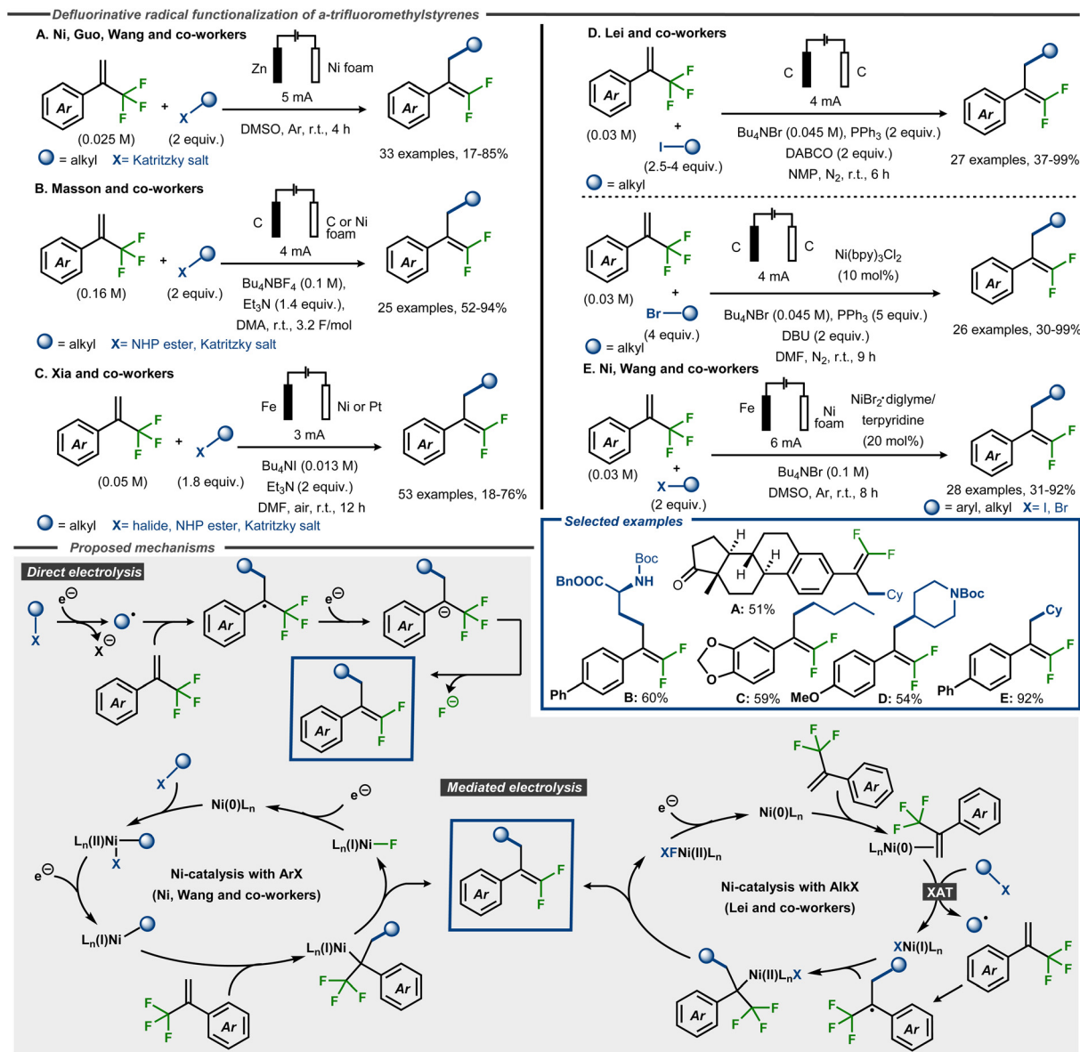
Fig. 18 Electoreductive formation of \gamma -functionalized gem -difluorostyrenes from \alpha -trifluoromethyl styrenes and radical precursors. 64–68
