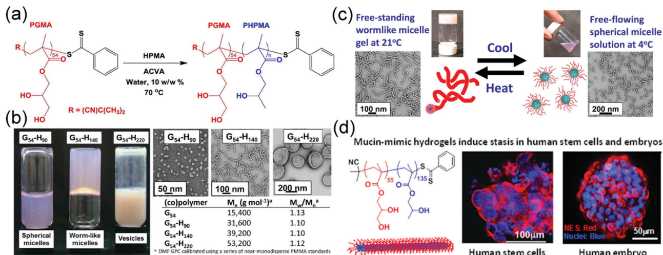
Fig. 19 (a) The synthesis and structure of PGMA–PHPMA polymer. (b) Digital photographs of three PGMA–HPMA copolymer dispersions (10 w/w%) at 21 °C, TEM images of diluted polymer solutions and molecular weight of the three polymers. (c) Thermo-induced morphology transformation of PGMA 54 –HPMA 140 assemblies. Reproduced with permission from ref. 253. Copyright 2012, American Chemical Society. (d) Structure of PGMA 55 –HPMA 135 polymer for wormlike thermogel and confocal image from 3D cell culture. Reproduced with permission from ref. 254 (DOI: 10.1021/acscentsci.5b00370). Copyright 2016, American Chemical Society.
