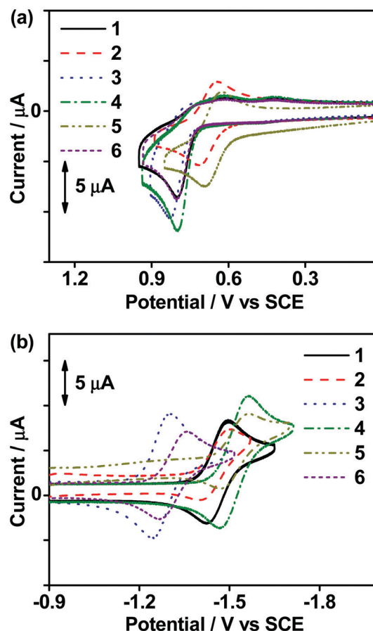
Fig. 1 Cyclic voltammograms for (a) oxidative and (b) reductive scans of 1–6 in degassed dichloromethane (0.1 M ^t\text{Bu}_4\text{NPF}_6 ) at 298 K.
