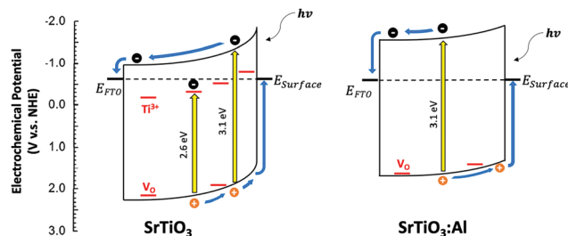
Fig. 12 Charge transfer and energetics during the SPV experiment for V_{\text{O}} rich \text{SrTiO}_3 and Al-doped \text{SrTiO}_3 (heating 1). In \text{SrTiO}_3\text{:Al} , \text{Ti}^{3+} trap states were eliminated by \text{Al}^{3+} doping, leading to a less reducing Fermi level, fewer trapped electrons, and less band bending. The lower band bending in \text{SrTiO}_3\text{:Al} is indicated by the lesser surface photovoltage signal. E_{\text{Surface}} denotes the energy of surface states resulting from dangling bonds, reduced ions, or surface adsorbates. \text{Ti}^{3+} and V_{\text{O}} lattice defects (shown in red) are responsible for the sub-band gap photovoltage signal. E_{\text{FTO}} is the Fermi level of the fluorine doped tin oxide substrate.
