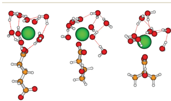
Fig. 11 Structures optimized in this work by DFT for the [\text{Pu}(\text{OH})_4\text{L}]^{n/m} complexes, with L = GTA (left), HBA (middle) and HIBA (right). n = -2 for GTA and m = -1 for HIBA and HBA. Colour code: Pu: green, O: red, C: orange, H: grey.
