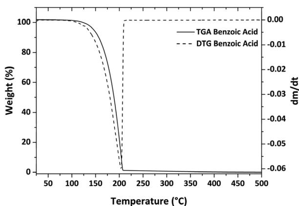
Fig. 2 Plot of the TGA/DTG analysis of benzoic acid.
