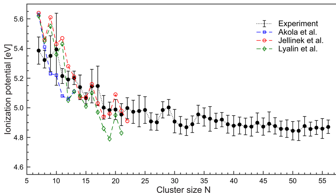
Fig. 4 Ionization potentials of \text{Mg}_N in the size range N = 7\text{--}56 (black \bullet ) extracted from the ionization efficiency curves. DFT-calculations on \text{Mg}_N have been conducted by Akola et al. 36 (blue \square ), Jellinek et al. 37 (red \circ ) and Lyalin et al. 38 (green \diamond ). Lines are used to guide the eyes.
