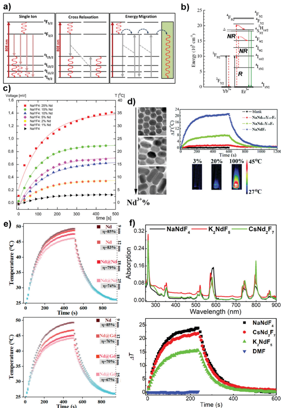
Fig. 7 (a) Simplified energy levels of \text{Nd}^{3+} ions and photophysical processes that lead to photothermal effect after 808 nm light irradiation. 70 Reprinted with permission from ref. 70. Copyright 2014, AIP Publishing LLC. (b) Simplified energy levels of \text{Yb}^{3+} and \text{Er}^{3+} ions, and photophysical processes after 975 nm light irradiation. 104 Reprinted with permission from ref. 104. Copyright 2009, The Optical Society. (c) Temperature change profiles of a cyclohexane solution of cubic phase NaYF 4 nanocrystals doped with \text{Nd}^{3+} (1–25%) excited using an 808 nm laser. 99 Reprinted with permission from ref. 99. Copyright 2011, Elsevier. (d) TEM images of NaYF 4 nanocrystals doped with different amounts of \text{Nd}^{3+} to illustrate the effects of dopant concentration on the morphology and photothermal performance of NaYF 4 : \text{Nd}^{3+} (3%, 20% and 100%) nanocrystals. 68 Reprinted with permission from ref. 68. Copyright 2019, Royal Society of Chemistry. (e) Effects of the thickness of NaNdF 4 (upper panel) and NaGdF 4 (lower panel) shells on the temperature change. 110 Reprinted with permission from ref. 110. Copyright 2020, American Chemical Society. (f) Absorption spectra of NaNdF 4 , K 2 NdF 5 and CsNd 2 F 7 nanocrystals (upper panel) and their corresponding temperature change profile (lower panel) obtained after being excited using an 808 nm laser. 107 Reprinted with permission from ref. 107. Copyright 2021, American Chemical Society.
