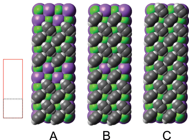
Fig. 3 Structure models A, B, and C for the system NaCl(100)/( 3\sqrt{2} \times \sqrt{2} ) R45^\circ - C_2H_2 with 4, 5, and 6 translationally inequivalent molecules per unit cell, respectively. Shown are 2 \times 2 unit cells in top view. The red square rectangle on the left illustrates the extension of the surface unit cell, while the dashed line indicates the reduced size of a ( \sqrt{2} \times \sqrt{2} ) R45^\circ cell. See also Table 1.
