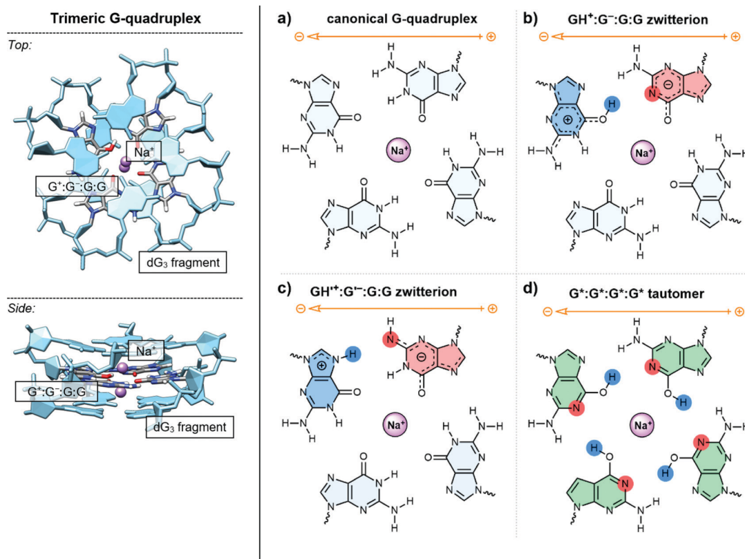
Fig. 4 Left: The trimeric G-quadruplex investigated by Jacquemin and Cerón-Carrasco, with the central quadruplex (depicted atomistically) shown in its G^+:G^-:G:G (oxonium/azanide) zwitterion form. Optimised structure taken from ref. 140. Right: Chemical structures of a canonical G-quadruplex, G^+:G^-:G:G (oxonium/azanide) and GH^+:G^-:G:G (iminium/azanide) zwitterion, and a G^*:G^*:G^*:G^* (quadruple enol/pyrimidine) rare tautomer. The direction of the EF required to induce these proton transfers is indicated by an orange arrow. Solid red circles indicate the deprotonated heteroatom, while solid blue circles indicate the transferring proton.
