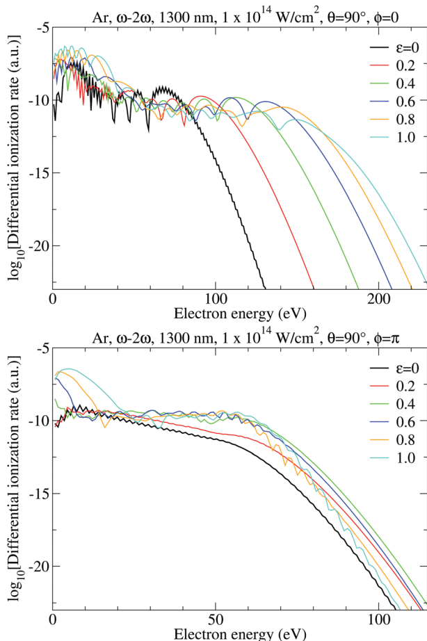
Fig. 7 The logarithm of the differential ionization rate of Ar atoms as a function of the photoelectron energy in electron volts for ionization by an \omega-2\omega BEOCT field with the ellipticities \varepsilon = \varepsilon_1 = \varepsilon_2 denoted in the panels. Both the direct and the rescattered electrons are included. The intensities of the field components are I_1 = I_2 = 1 \times 10^{14} \text{ W cm}^{-2} , the fundamental wavelength is 1300 nm, and emission is in the direction of the semi-minor axis of the polarization ellipse ( y axis). The relative phase is \phi = 0 (upper panel) and \phi = \pi (lower panel).
