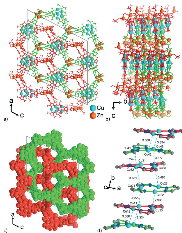
Fig. 8 View along the hexagonal channels of the two interpenetrating 3D-frameworks in 3 as (a) and (b) wire-frame, and (c) space-filling modes. Network A in red with the Zn_3 -SBU and network B in green with the Zn_4 -SBU (cf. Fig. 7). (d) Stacking of the \{Cu_3(pz)_3\} moieties in 3 with Cu^I \cdots Cu^I contacts (in cyan, distances in Å) between the layers of the interpenetrating frameworks.
