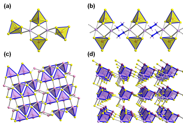
Fig. 5 Molecular structure of the [Mn_2As_4S_{16}]^{8-} cluster anion (a), fragment of the 1D- \{[Mn_2As_2S_8(N_2H_4)_2]\}^{6-} strand formed from \mu - N_2H_4 -linked [Mn_2As_2S_8]^{6-} clusters (b), view of the 2D- \{[Cu_3As_2S_5]^{-}\} layer (c) and the open-framework constructed by [MnAs_3S_6]^{-} clusters (d). Counterions are omitted for clarity. Color code: As-plum, Mn-lavender, Cu-rose, S-yellow, N-blue.
