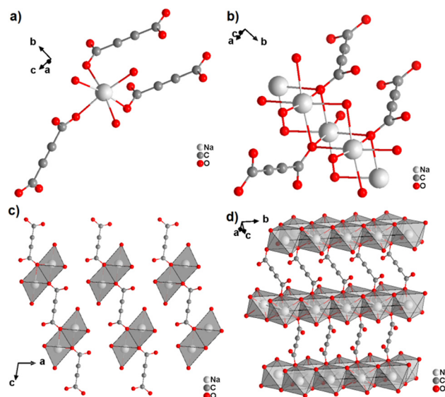
Fig. 5 Crystal structure of hydrated sodium acetylenedicarboxylate [ \text{Na}_2(\text{ADC})(\text{H}_2\text{O})_4 ] showing: (a) the coordination environment of the Na atom, (b) the coordination mode of ADC linkers and water oxygen atoms, and (c) and (d) sheets from chains of \text{NaO}_6 octahedra connected by ADC linkers. Graphics redrawn from the cif file (CSD-Refcode XADSAX). 42
