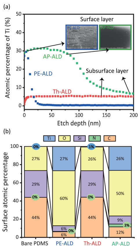
Fig. 2 (a) XPS depth profiling showing the atomic percentage of titanium in the surface and subsurface of various PDMS samples and (b) XPS elemental analysis of the surface. All depositions were conducted at 100 °C for 100 cycles, and the \text{TiO}_x layer thickness is estimated to be 7 and 78 nm for the PE-ALD and AP-ALD treated samples, respectively.
