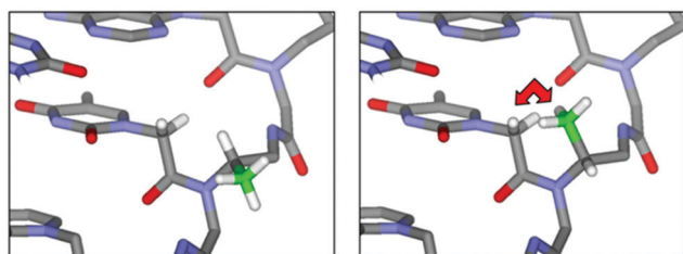
Fig. 5 A model of the \beta PNA structure showing a different degree of steric clash between the \beta -( S )- or \beta -( R )-methyl groups and the nucleobase side arm (reprinted from ref. 36, Copyright (2011), with permission from Elsevier).
