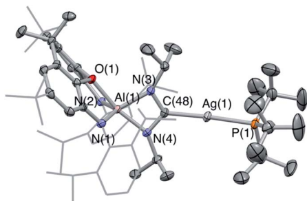
Fig. 4 Molecular structure of 5-Ag in the solid state as determined by X-ray crystallography. Thermal ellipsoids set at the 50% probability level. Hydrogen atoms omitted and ^1\text{Pr}/^t\text{Bu} shown in wireframe for clarity. Key bond lengths (Å) and angles ( ^\circ ): Ag(1)–C(48): 2.118(2), Ag(1)–P(1): 2.3851(6), N(3)–C(48): 1.346(3), N(4)–C(48): 1.345(3).
