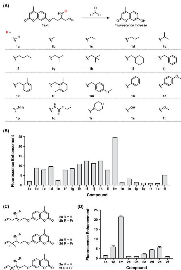
Fig. 2 Screening and comparison of various self-immolative aza-Cope reaction-based coumarin probes for determining optimal aza-Cope reactivity of FA. (A) Chemical structures of aza-Cope-based coumarin probes with varying N -substituents synthesized in this study. (B) Screening of coumarin probes shown in (A) by fluorescence enhancement of the probes toward FA. (C) Chemical structures of aza-Cope-based coumarin probes with additional methyl groups. (D) Comparison of the N -substituent effect with the gem -dimethyl effect on aza-Cope reactivity by fluorescence enhancement of the probes toward FA. Probe (10 \mu M) was treated with 1 mM FA in PBS (20 mM, pH 7.4) at 37 ^{\circ} C for 2 h. The fluorescence intensity at 445 nm was recorded with excitation at 317 nm. Data are shown as mean fluorescence enhancement after versus before FA treatment \pm standard deviation ( n = 3 ).
