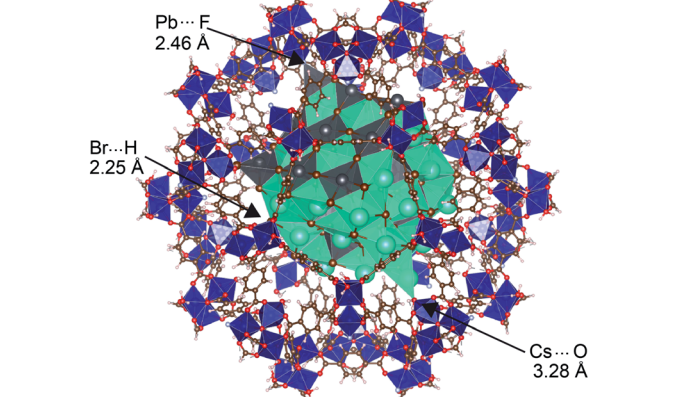
Fig. 6 Electronic density of states calculated for (a) Cr-MIL-101 and (b) nano CsPbBr 3 . (c) Minimum-energy geometry for CsPbBr 3 @nano-Cr-MIL-101.
