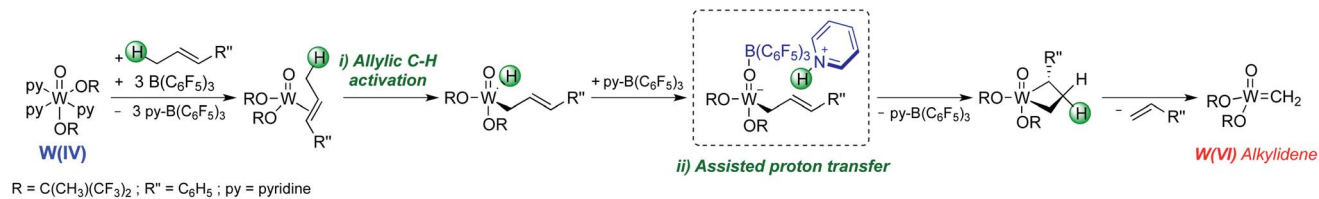
Scheme 9 Proposed initiation mechanism for W(IV) oxo complex [W(OtBuF_6)_2(py)_3] .
