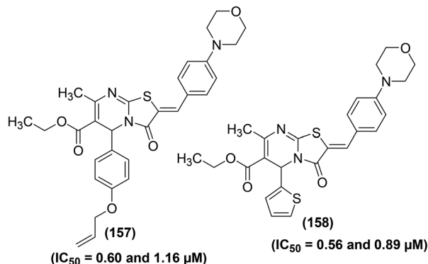
Fig. 49 Chemical structures of selected thiazolo[3,2-a]pyrimidines (157 and 158).
