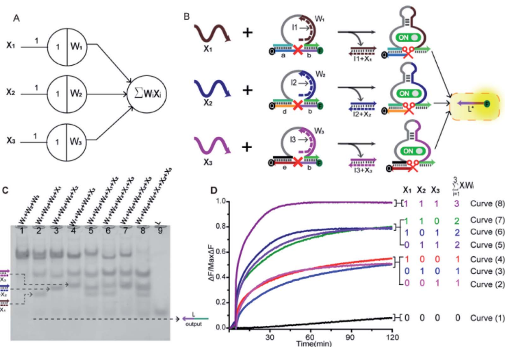
Fig. 3 (A) Abstract diagram of the three-input integration gate motif and its DNA implementation. The black numbers indicate the initial relative concentration. (B) Illustration of the integration gate. The inputs signal consisted of three parts: X_1 , X_2 and X_3 ; the weights consisted of three parts: W_1 , W_2 and W_3 . All substrate strands ( S_{1a,b} , S_{2d,b} , S_{3e,b} ) were labelled with fluorophore FAM at 5'-end and quencher BHQ1 at 3'-end for fluorescent signal determination; L^* was the normalized output. (C) Native PAGE analysis of the integration gate. The strands and complex involved were labelled above the lane number. Lane 1, weight unit mixture ( W_1 + W_2 + W_3 ); lane 2, X_1 was added to the weight unit mixture; lane 3, X_2 was added to the weight unit mixture; lane 4, X_3 was added to the weight unit mixture; lane 5, X_1 and X_2 were added to the weight unit mixture; lane 6, X_1 and X_3 were added to the weight unit mixture; lane 7, X_2 and X_3 were added to the weight unit mixture; lane 8, all signals were added to the weight unit mixture; lane 9, normalized product strand L . (D) Normalized fluorescence of the integration gate. The standard concentration was 1 \times 0.2 \mu\text{M} , [W_1] : [W_2] : [W_3] : [X_1] : [X_2] : [X_3] = 1 : 1 : 1 : 1 : 1 : 1 . The sum value was inferred from the fluorescent signal. Curve (1) had no input signals added; Curves (2)–(4) had only one input signal added; Curves (5)–(7) had two kinds of input signals added; Curve (8) had all input signals added.
