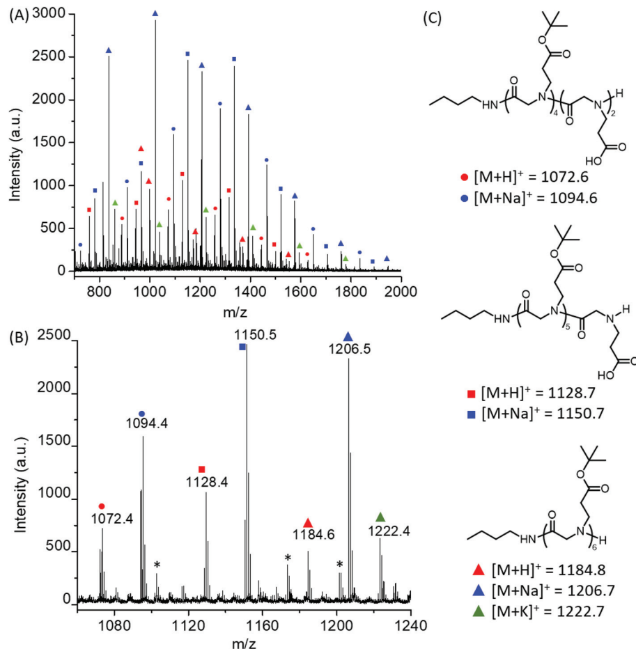
Fig. 2 (A) Full and (B) expanded MALDI-TOF MS spectrum of a low molecular weight poly( N -(3- tert -butoxy-3-oxopropyl) glycine) obtained from the butylamine-initiated ROPs of t BuO 2 Pr-NCA in toluene together with (C) the structural assignment of the molecular ions and corresponding calculated m/z values. * ( m/z = 1101.7, 1173.4 and 1201.4) correspond to poly( N -(3- tert -butoxy-3-oxopropyl) glycine) species whose end-group structures are presently unclear.
